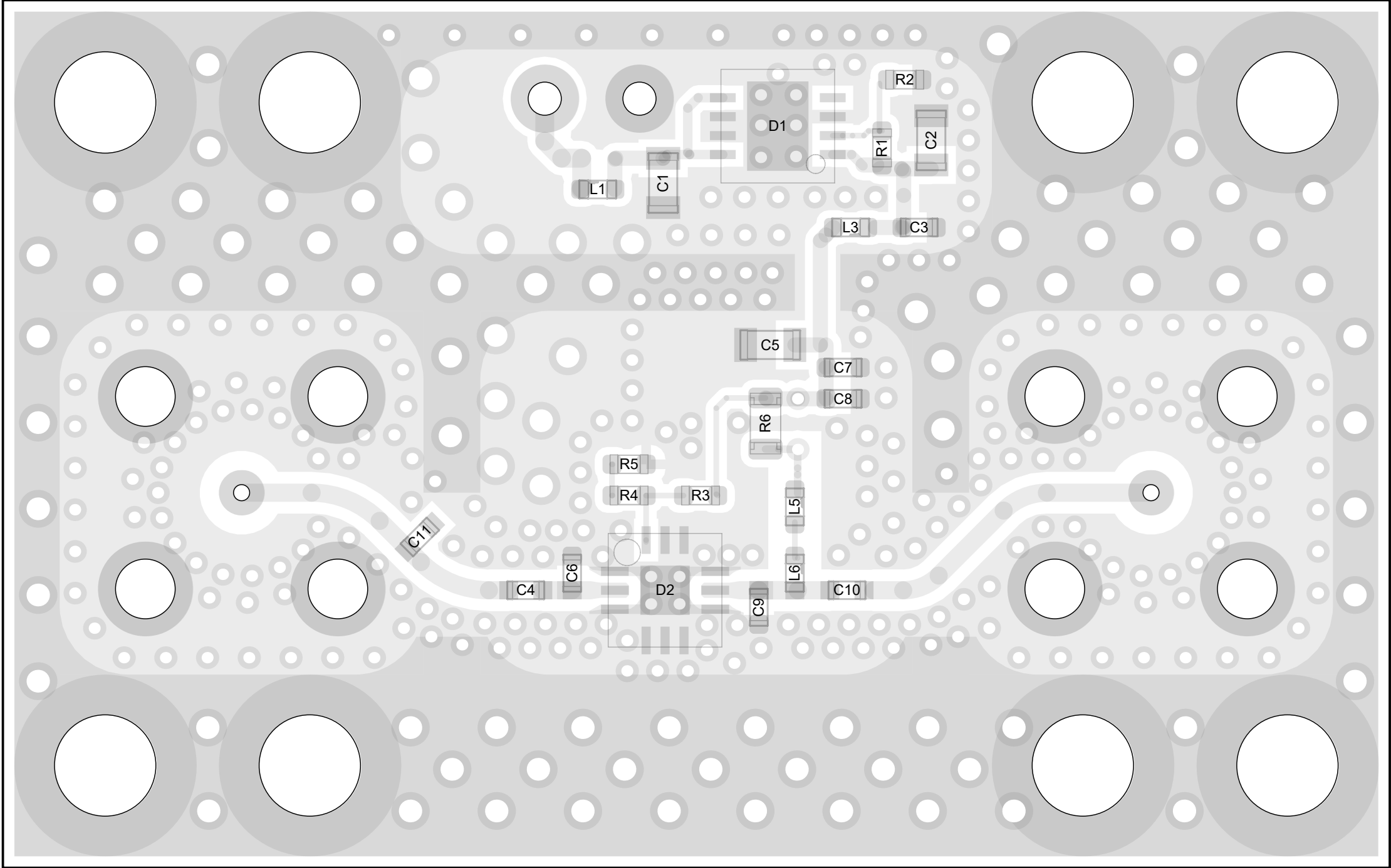
View from Top side (Scale 8:1)
