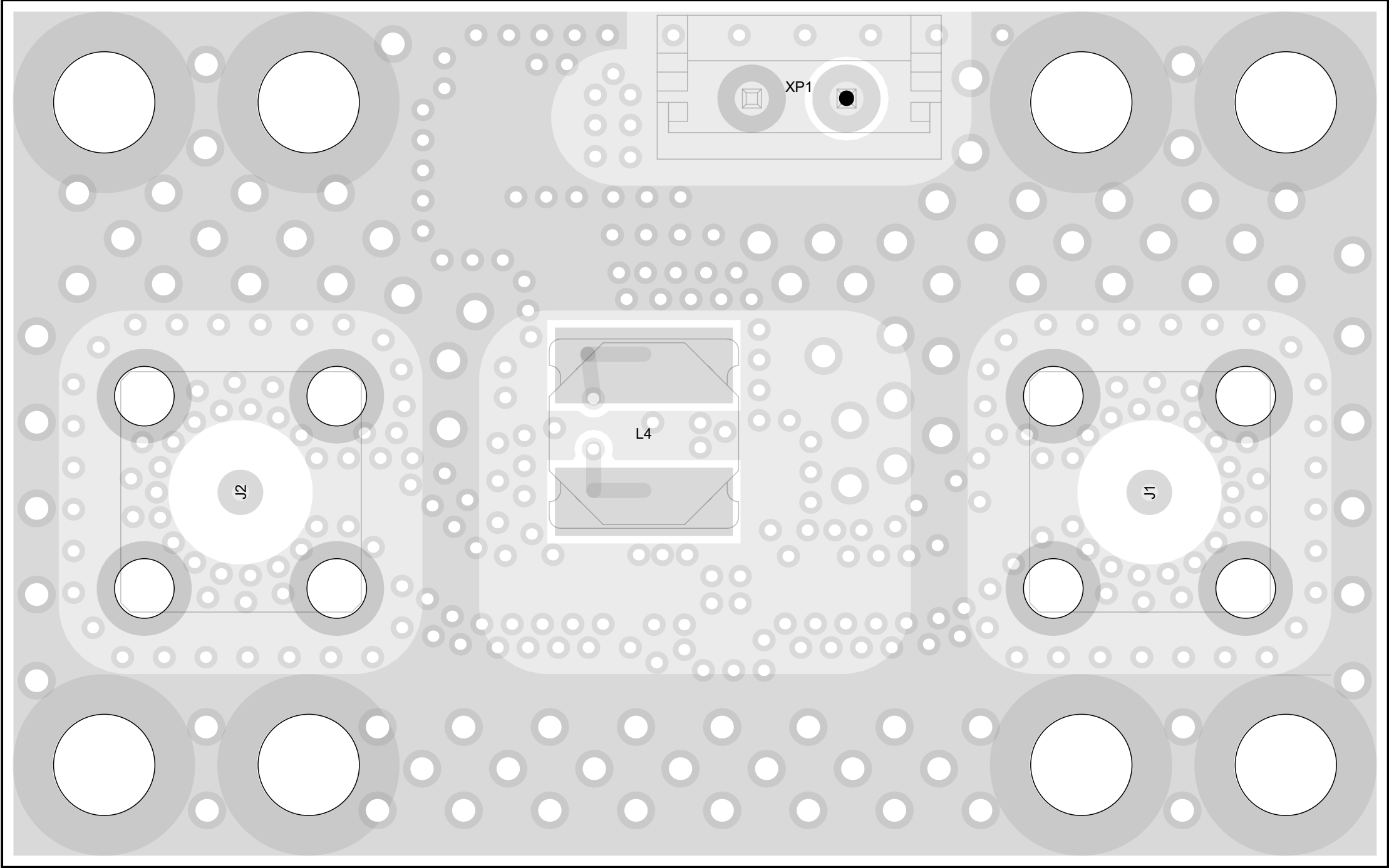
View from Bottom side (Scale 8:1)
